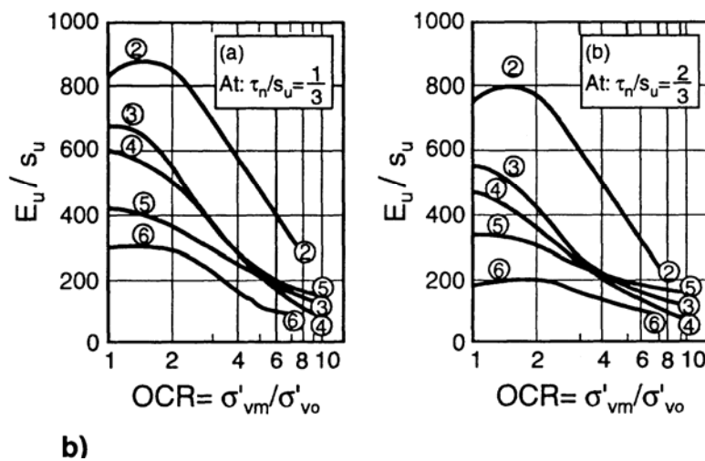
Figure 39 Selection of soil stiffness ratio for clays (after Ladd et al., 1977)
