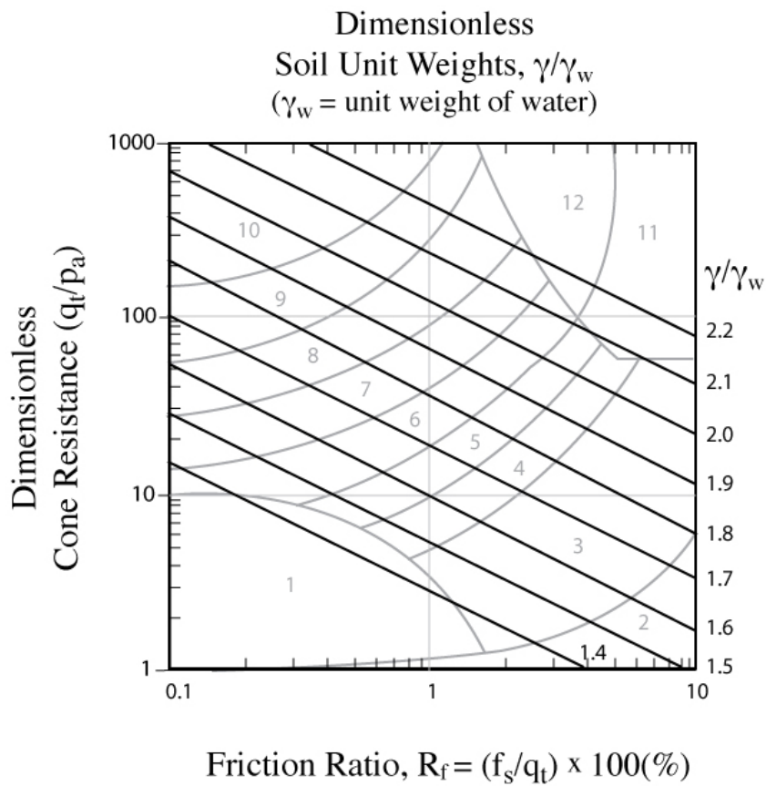
Figure 26 Dimensionless soil unit weight, \gamma/\gamma_w based on CPT
