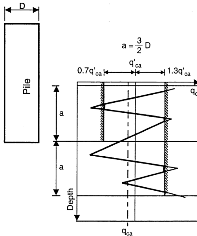
Figure 40 Calculation of equivalent average cone resistance (Bustamante and Gianselli, 1982).
