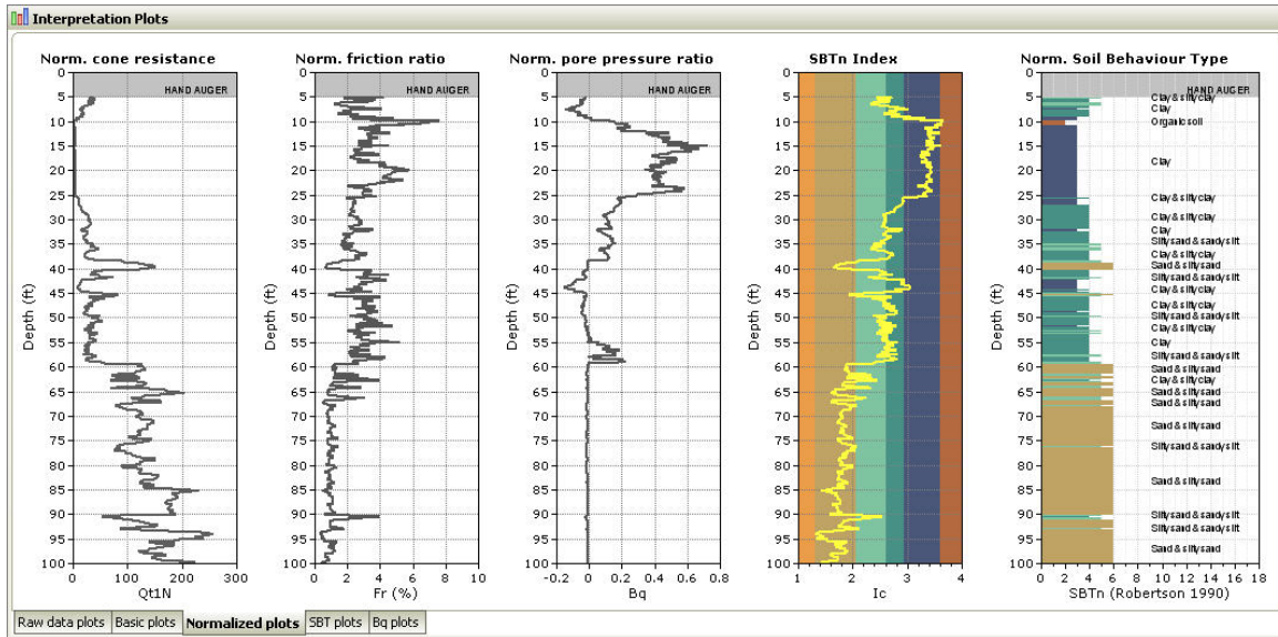
Figure 50 Example CPTu plot based on normalized parameters from CPeT-IT
