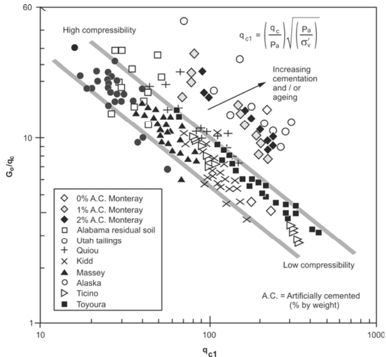
Figure 31 Characterization of uncemented, unaged sands (after Eslaamizaad and Robertson, 1997)
